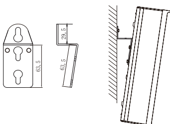
Wall hanging bracket (accessories)
